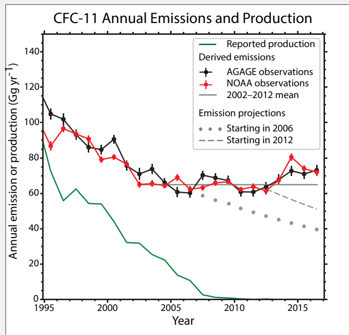
Figure ES-2. CFC-11 global emissions and reported production.
